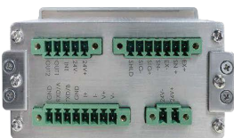
RS485/232 + Analog output
